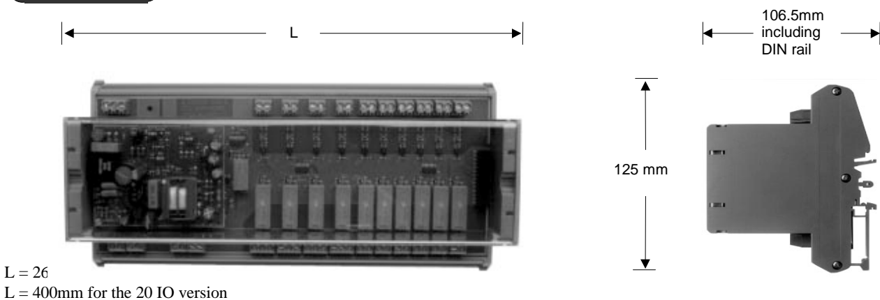
Figure 1-2: Dimensions
