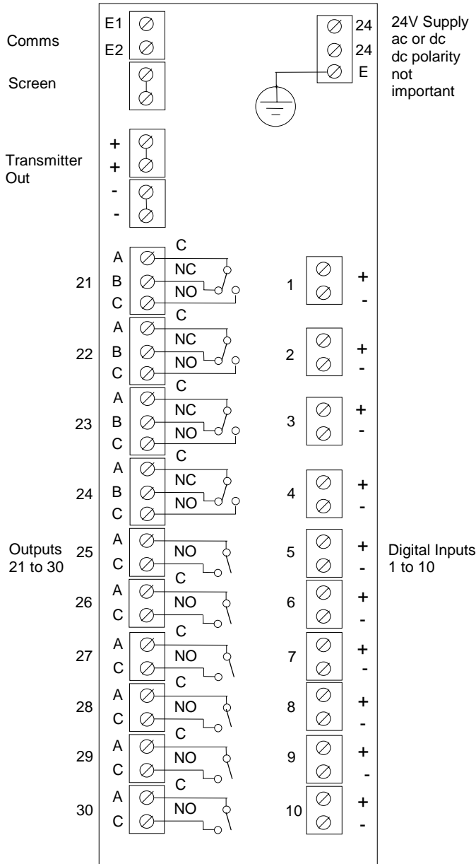
Figure 1-3: 10 Input/10 Output IO Expander Terminals
