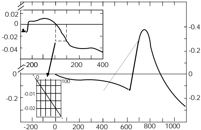
Figure 1 The temperature difference (t_{90} - t_{68})/^{\circ}\text{C} in the range between the triple point of equilibrium hydrogen ( -259.3467^{\circ}\text{C} ) and the freezing point of gold ( 1064.18^{\circ}\text{C} ) [83.85]
